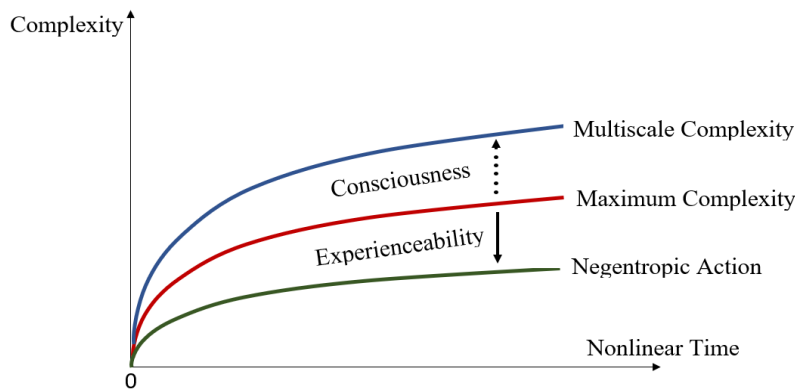
Figure 3. Functionality can be decoded from the structure of intrinsic information. It arises from the complexity versus nonlinear time because nonlinear time dampens the increasing entropy production and increases multiscale complexity. The addition to the maximum complexity (red) of “potential complexity” due to systems patterns of experienceable forms by the process of negentropic action (Green) reduces the maximum complexity in systems with internal constrictions (heterogeneous dissipative systems) to produce qualitatively novel aggregativity, leading to new systemic qualities expressed as functionality. Functionality underlying intrinsic intentionality can reduce functionality below maximum complexity (Green). Moreover, negentropic entanglement increases the functionality of maximum complexity, referred to as “multiscale complexity” (blue), but in return, also instantiates consciousness. This suggests that through negentropic entanglement, a weak unity of consciousness is made possible by the contiguity of “potential complexity”. There appears to be a gradual increase in the functionality of multiscale complexity.
